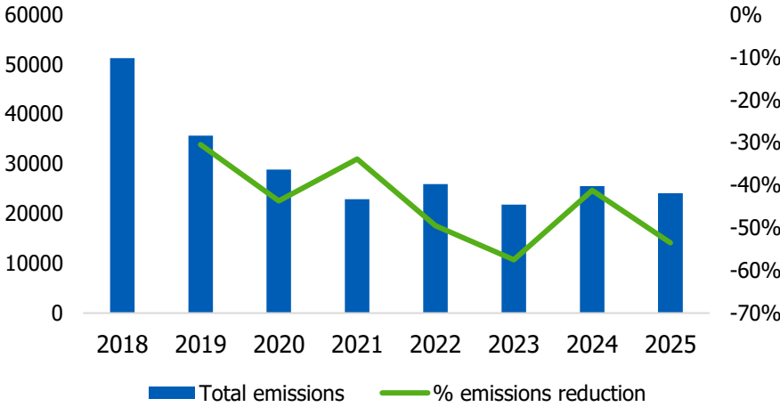
Evolution of total emissions (t CO2e)
